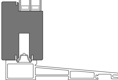
Sill
